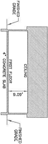
SECTION C-C
